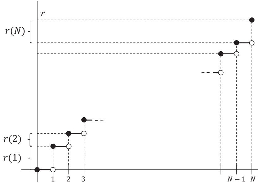
Figure 6.6: Function F defined by (6.48).
