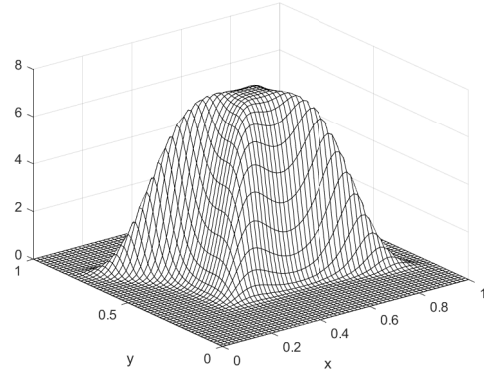
Figure 6.2: Optimal probability density Q^*(x) .
