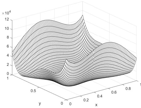
Figure 6.1: Surface plot of C(x) .
