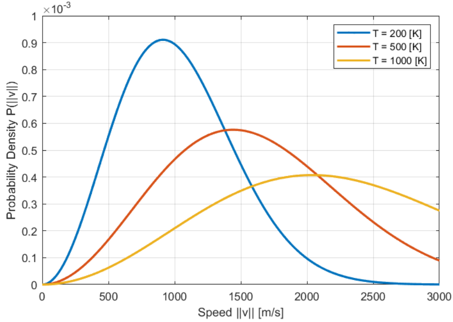
Figure 6.4: Maxwell-Boltzmann speed distribution of Helium gas.
