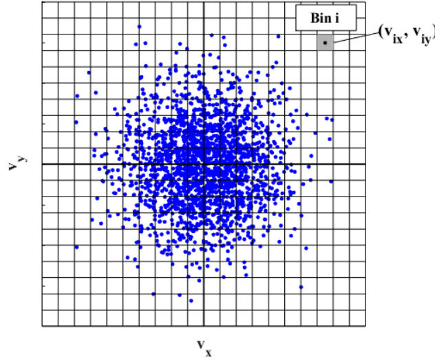
Figure 6.3: Maxwell velocity distribution.
